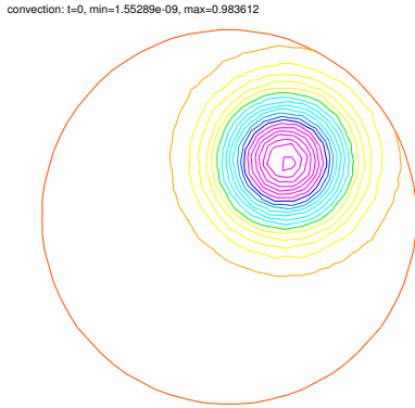
Figure 9.20: u^0 = e^{-10((x-0.3)^2+(y-0.3)^2)}
