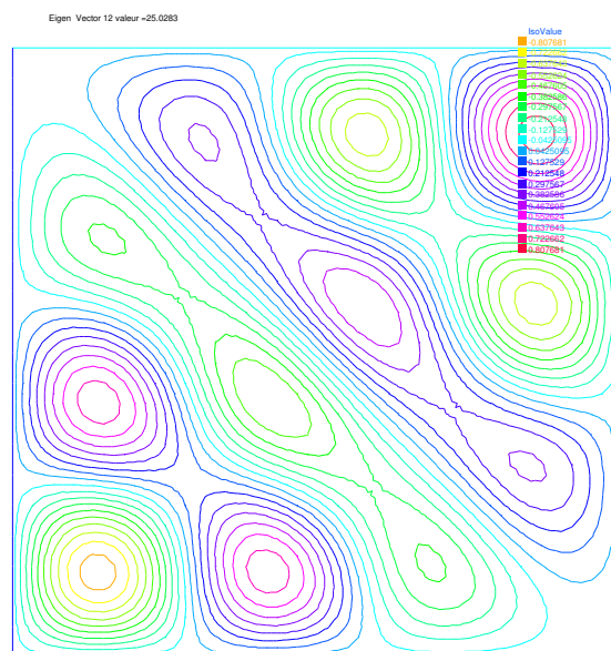
Figure 9.18: Isovalue of 12th eigenvector u_{4,3} + u_{3,4}
