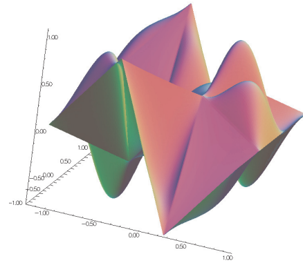
Figure 6.7: projection to V_h(\mathcal{T}_h, \mathbf{P1b})
