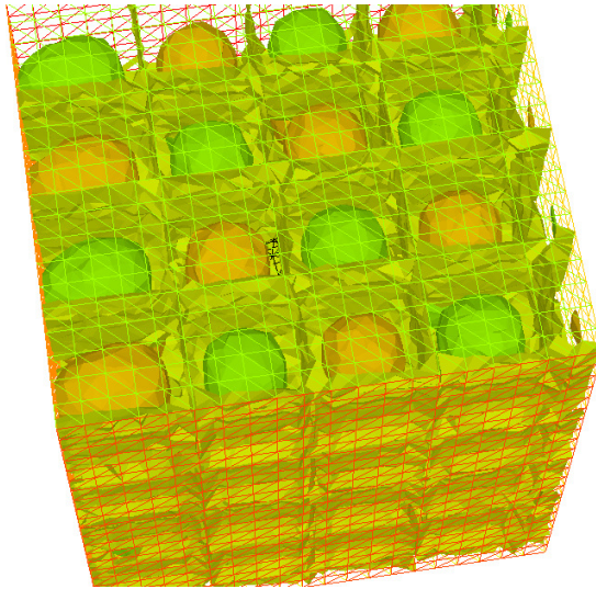
Figure 9.9: view of the surface isovalue of periodic solution u_h
